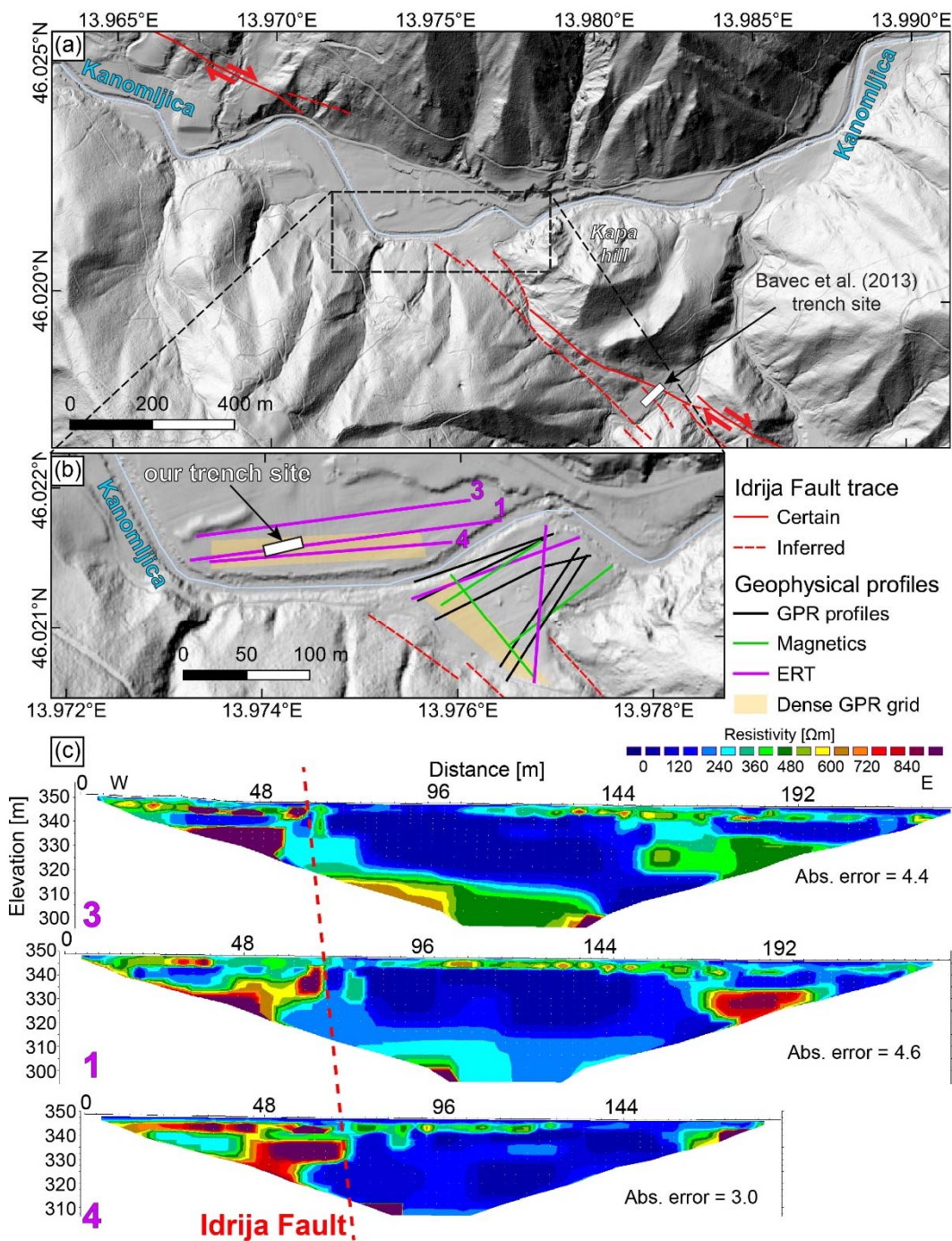
355 Figure 10: Map of the trench site at the Idrija Fault and selected ERT data. (a) Setting of the trench site and mapped traces of the Idrija Fault after Cunningham et al. (2006), Bavec et al. (2013), and Moulin et al. (2014). The precise fault trace is unknown in the flood plain of the Kanomljica River. (b) Detailed view of the location of all geophysical profiles used for trench site selection. (c) ERT profiles 1, 3, and 4 that were crucial for trench site location. Red dashed line indicates the interpreted fault trace. All data show
