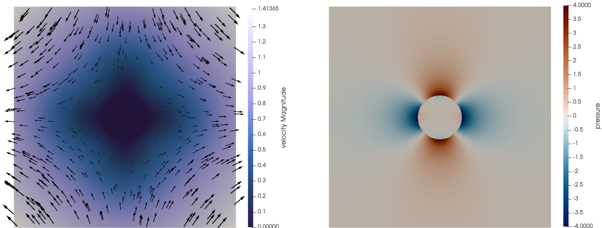
Figure 6. SolVi benchmark with inclusion of radius 0.2. Velocity (left) and pressure (right) fields obtained on a 256 \times 256 mesh using Q_2 \times Q_1 elements.
