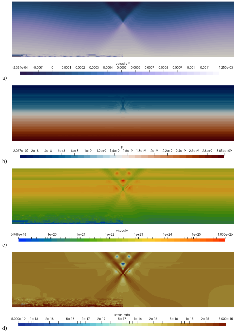
Figure 13. Application example. a) Vertical component of the velocity field; b) pressure field; c) Effective viscosity field; d) Effective Strain rate field. In all figures, the left half (left of the vertical line) shows data obtained with the stabilised Q_1 \times Q_1 element, whereas the right half shows results obtained with the Q_2 \times Q_1 element. Note the large deviations between the two towards the bottom of the domain. All results were obtained on an 800 \times 200 mesh with a cell size of 0.5 km.
