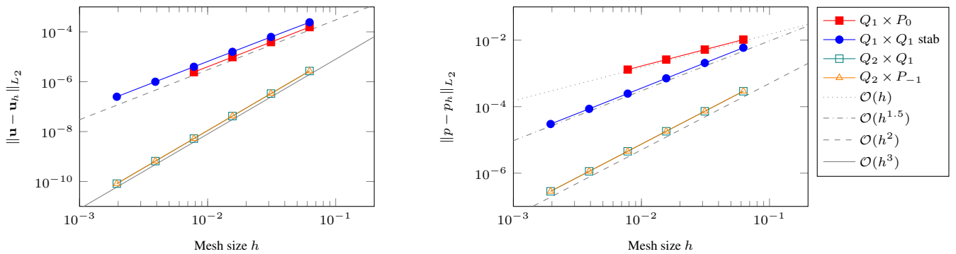
Figure 2. Donea & Huerta benchmark. Error convergence as a function of the mesh size h . Left: Velocity error \|\mathbf{u} - \mathbf{u}_h\|_{L_2} . Right: Pressure error \|p - p_h\|_{L_2} . The two leftmost points are missing for Q_1 \times P_0 since the solver failed to converge; the data points for Q_2 \times Q_1 and Q_2 \times P_{-1} are on top of each other.
