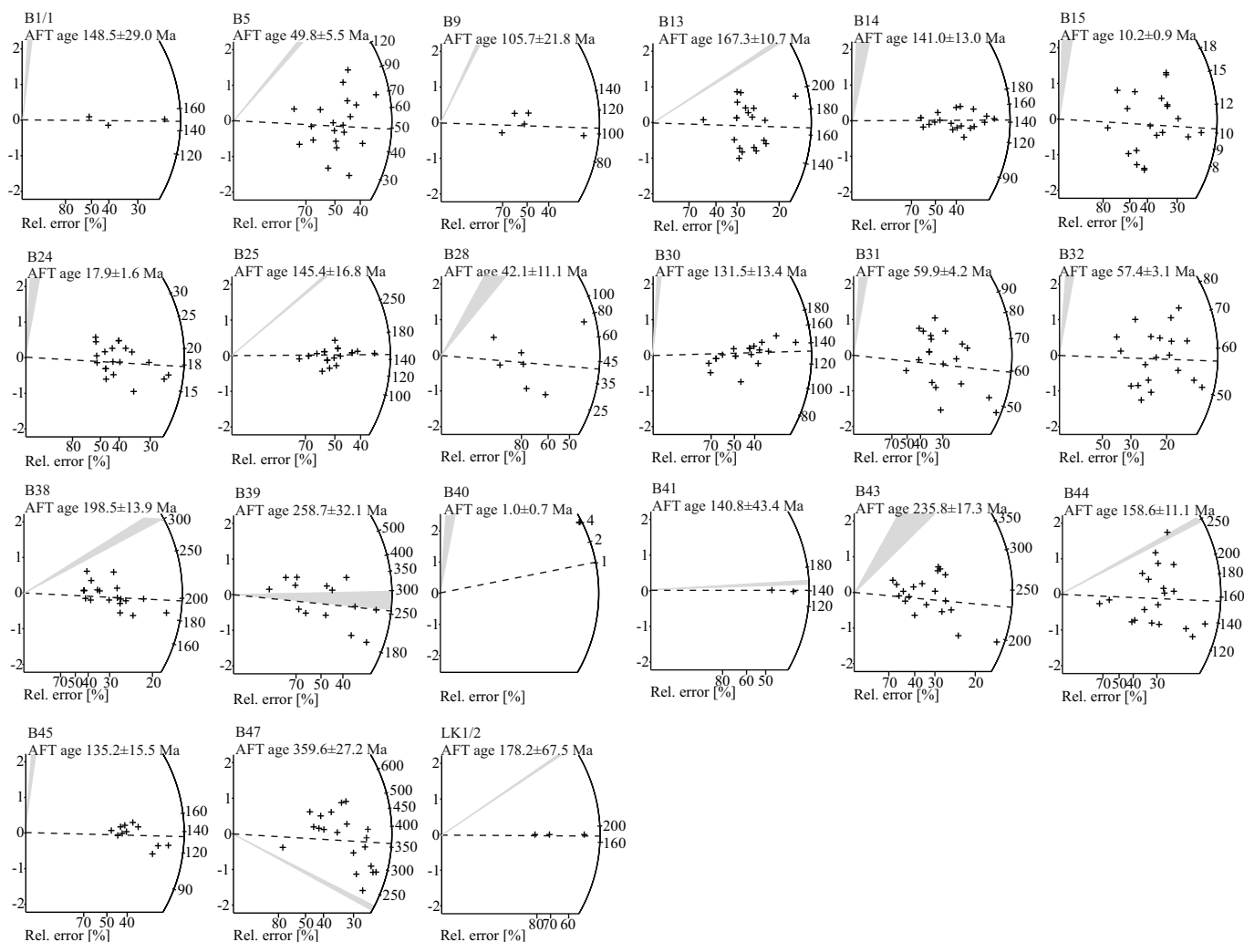
Figure A1. Radial plots of apatite fission track data. Central ages of samples are defined by dashed lines, stratigraphic ages are represented by shaded areas. The position of the x-scale records the uncertainty of individual age estimates, whilst each point has the same standard error on the y-scale (illustrated as \pm 2\sigma ). The age of each crystal can be determined by a line from the origin through the projection point of the crystal to the intercept on the radial age scale (Galbraith, 1990)
