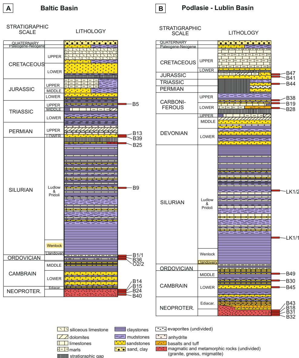
Figure 3. Simplified chronostratigraphic logs for the Podlasie-Lublin and Baltic Basins with the location of samples indicated (based on various sources including Żelichowski, 1987; Modliński et al., 2010; Poprawa, 2010)
