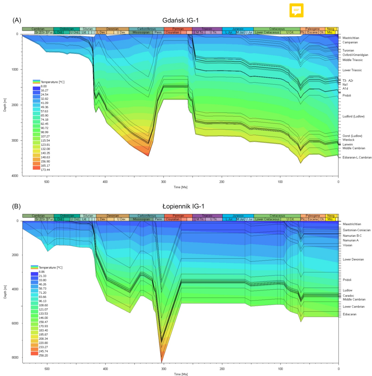
Figure 5. Representative burial history plots for (A) Baltic Basin, and (B) Lublin Basin after Botor et al. (2019a). In the Baltic and Lublin Basins, a maximum temperature in the lower part of the Ediacaran-Palaeozoic sedimentary succession was reached in the early and latest Carboniferous, respectively.
