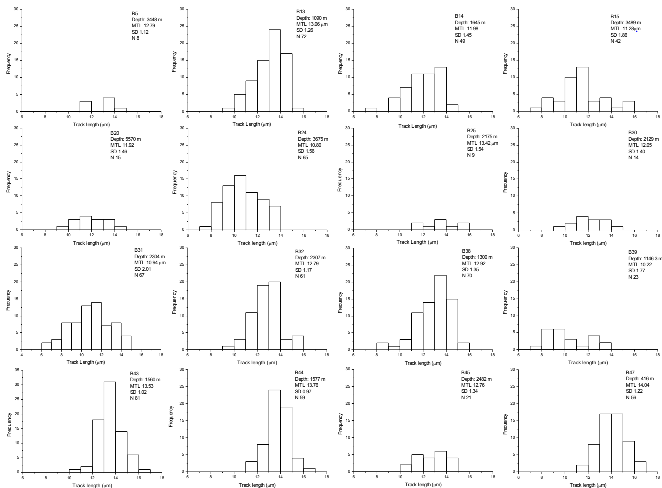
Figure A2. Length distributions of confined fission tracks in analysed samples.
