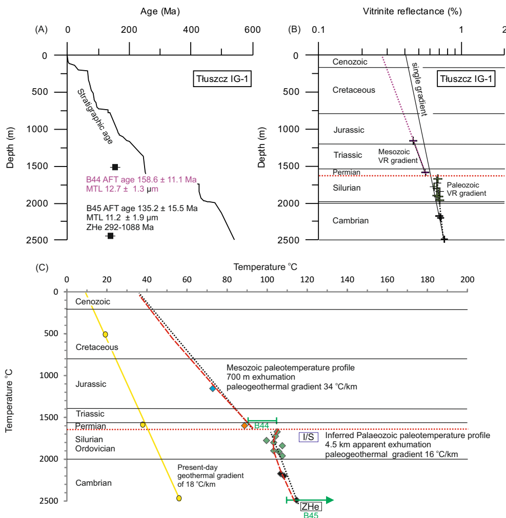
Figure 9. Tluszcz IG-1 borehole data (Podlasie Basin). (A) Thermochronological data vs stratigraphic age, (B) VR profile, (C) paleotemperature profile. Note a thermal maturity break at the unconformity between the Permian-Mesozoic and Silurian. The Mesozoic paleotemperature profile shows 700 m of exhumation with a paleogeothermal gradient of 34 ^{\circ} C/km. The inferred Palaeozoic paleotemperature profile shows 4.5 km of apparent exhumation with a paleogeothermal gradient of 16 ^{\circ} C/km. A nonlinear VR profile suggests a fluid flow event. Other explanations as in Figures 6 and 7. Illite K-Ar ages from Silurian bentonites are 334-311 Ma (mid-late Carboniferous) in the adjacent Goździk OU-1 well (Kowalska et al., 2019)
