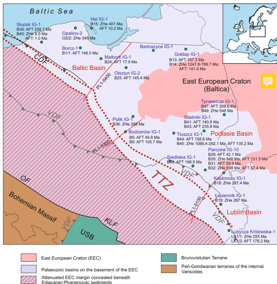
Figure 1. Simplified tectonic map of central and north-eastern Poland (modified from Mazur et al., 2018b) showing the location of samples and the AFT and ZHe ages obtained. Location of PolandSPAN TM seismic profiles (PL1-5100, 5300, 5400) used in Figure 2 is indicated. CDF - Caledonian Deformation Front; KLF - Kraków-Lubliniec Fault; OF - Odra Fault; VDF - Variscan Deformation Front; TTZ - Teisseyre-Tornquist Zone; USB - Upper Silesia Block.
