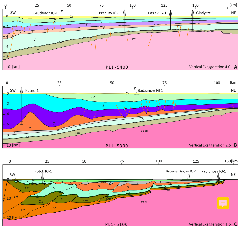
Figure 2. Vertically exaggerated geological sections across the south-western slope of the East European Platform, showing the structure of sedimentary cover and top of the crystalline basement. Cross-sections are built upon the PolandSPAN TM seismic profiles PL1-5400 (A), PL1-5300 (B) and PL1-5100 (C) for the Baltic, Podlasie and Lublin Basins, respectively. Modified from Mazur et al. (2018a); (A) and Mazur et al. (2015); (B) and (C). Abbreviations of chronostratigraphic units: Pcm - Paleoproterozoic; Ed - Ediacaran; Cm - Cambrian; Or - Ordovician; S - Silurian; D - Devonian; C - Cambrian; P - Permian; T - Triassic; J - Jurassic; Cr - Cretaceous; Cz - Cenozoic.
