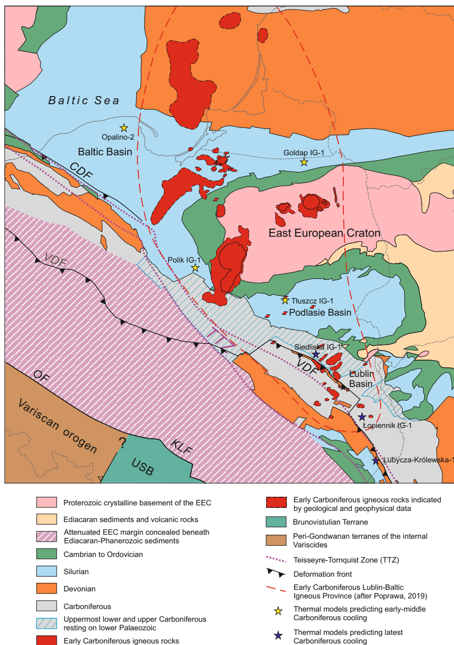
Figure 14. Pre-Permian geology map for the SW slope of the East European Platform in Poland and adjacent areas. The extent of early Carboniferous igneous rocks and the Lublin-Baltic Igneous Province is shown after Poprawa (2019). Location of the Variscan Deformation Front is from Mazur et al. (2020). Further explanations in the text. CDF - Caledonian Deformation Front; KLF - Kraków-Lubliniec Fault; OF - Odra Fault; TTZ - Teisseyre-Tornquist Zone; USB - Upper Silesia Block; VDF - Variscan Deformation Front.
