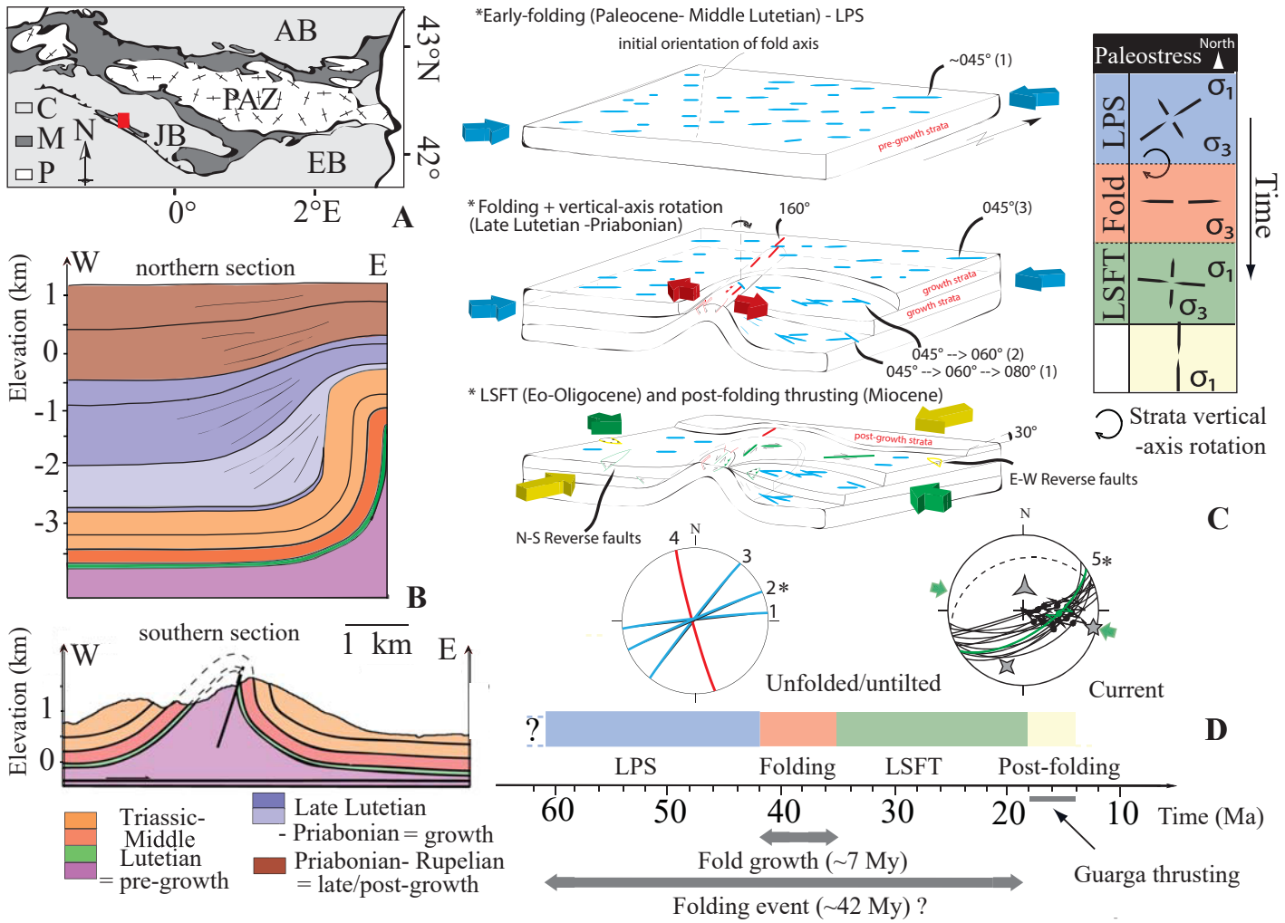
Fig.5. Pico del Aguila anticline: A: location (AB: Aquitaine Basin, JB: Jaca Basin, EB: Ebro Basin, PAZ: Pyrenean Axial Zone; P: Paleozoic; M: Mesozoic; C: Cenozoic). B: Cross sections (north : modified after Poblet et al., 1997, south : modified after Beaudoin et al., 2015). C: Orientation of the main sets of mesostructures (relative chronology, 1 to 5), reported in current or unfolded attitude on a lower hemisphere Schmidt stereonet (same key as Fig.3), and associated structural and paleostress evolution. Block diagrams modified after Beaudoin et al. (2015). * denotes mesostructures dated using U-Pb. D: Timing and duration of deformation stages. Color code for C and D : blue: layer-parallel shortening (LPS); red: fold growth; green: late stage fold tightening (LSFT); yellow: post-folding compression.
