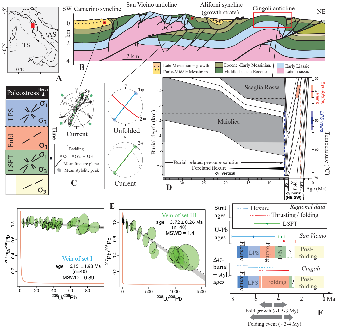
Fig.3. San Vicino and Cingoli anticlines: A: location (AS: Adriatic Sea; TS: Tyrrhenian Sea). B: Cross section (modified after Mazzoli et al., 2002). C: Orientation of the main sets of mesostructures (relative chronology, 1 to 3), reported in current or unfolded attitude on a lower hemisphere Schmidt stereonet, and associated paleostress evolution. * denotes mesostructures dated using U-Pb. D: Burial model of Cingoli constructed considering thickness from stratigraphic and well data corrected for chemical and physical compaction (modified after Labeur et al., 2021). The range of depths reconstructed from sedimentary stylolite roughness inversion (with uncertainty shaded in light grey) are reported for each formation as grey levels. The results of clumped isotope analysis (i.e., temperatures of precipitation of vein cements at thermal equilibrium with the host rock) are reported for LPS-related veins (blue) and syn-folding veins (red). The deduced timing of the deformation stages is reported. E: Age dating results for veins from San Vicino anticline: Tera-Wasserburg concordia plots for carbonate samples showing ^{238}\text{U}/^{206}\text{Pb} vs ^{207}\text{Pb}/^{206}\text{Pb} for veins of sets I (LPS-related) and III (LSFT-related) (n—no. of spots). MSWD—mean square of weighted deviates. F: Timing and duration of deformation stages. Regional data are from Mazzoli et al., 2002 (flexure), Calamita et al. 1994 (folding and thrusting), Beaudoin et al., 2020c (LSFT). Color code for C and F: dark blue: flexure-related extension. blue: layer-parallel shortening (LPS); red: fold growth; green: late stage fold tightening (LSFT); yellow: post-folding extension.
