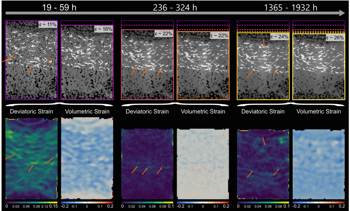
Figure 10. Locally resolved strain in the SB sample . The absolute values of deviatoric and volumetric strain were calculated from digital volume correlation for three different time steps. The top row shows the two microtomography scans which were compared to each other using digital volume correlation. Further, the contours are showing the sample dimensions, ranging in colour from purple for the least compacted sample to light yellow for the most compacted sample . In the bottom row, the results of the strain calculation are displayed. Note that the strains are cummulative-cumulative and cover the entire time interval between the two selected scans. The time intervals increase from the left to the right and are 40 hrs, 88 hrs and 567 hrs. For the deviatoric strain bright colours represent high strains whereas dark colours represent low strains. For the volumetric strain blue indicates compaction while red indicates dilation. Note the larger scale for the first time step of the deviatoric strain and that the strains are resolved on the grain scale. Arrows point to high deviatoric strains at NaCl-biotite interphase boundaries .
