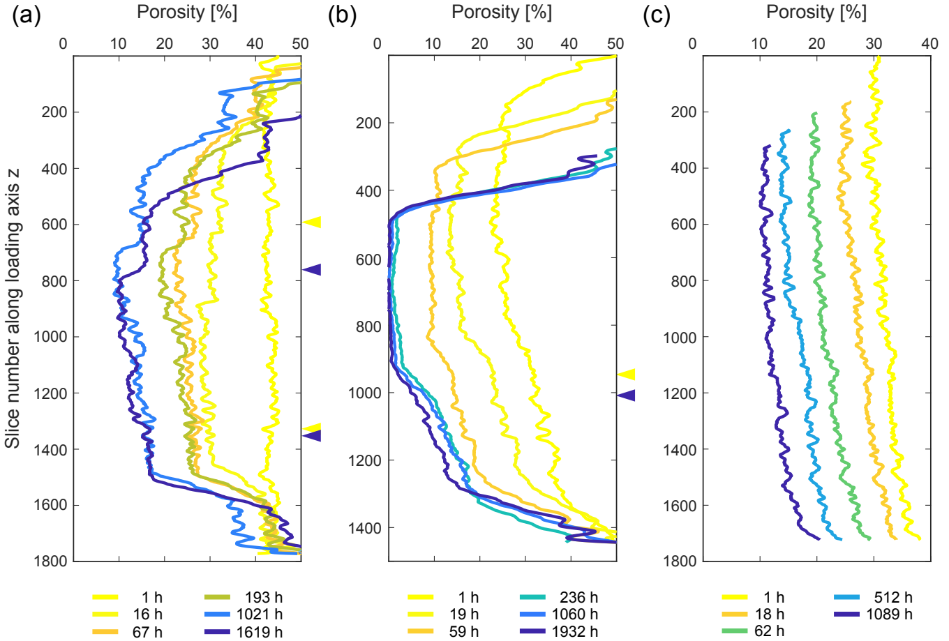
Figure 13. Porosity evolution of a) the pure NaCl, SBS b) the SB sample and c) the SBS pure NaCl sample with progressing deformation. The porosity was measured as 2-dimensional porosity for each slice along the loading axis. Different colours indicate different time steps, ranging from yellow to blue with progressing compaction. While a) shows a homogeneous decrease of the porosity within the sample , heterogeneities arise in b) and c) which show the compositionally layered samples, a) shows a homogeneous decrease of the porosity within the sample . The highest porosity loss occurs in biotite-bearing layers, resulting in compartmentalisation of the SB sample (cf. Sect. 2.5). Note that the arrows on the right hand side mark the transition from the pure NaCl domain to the NaCl-biotite domain and colours are corresponding to the deformation stage as denoted in the key.
