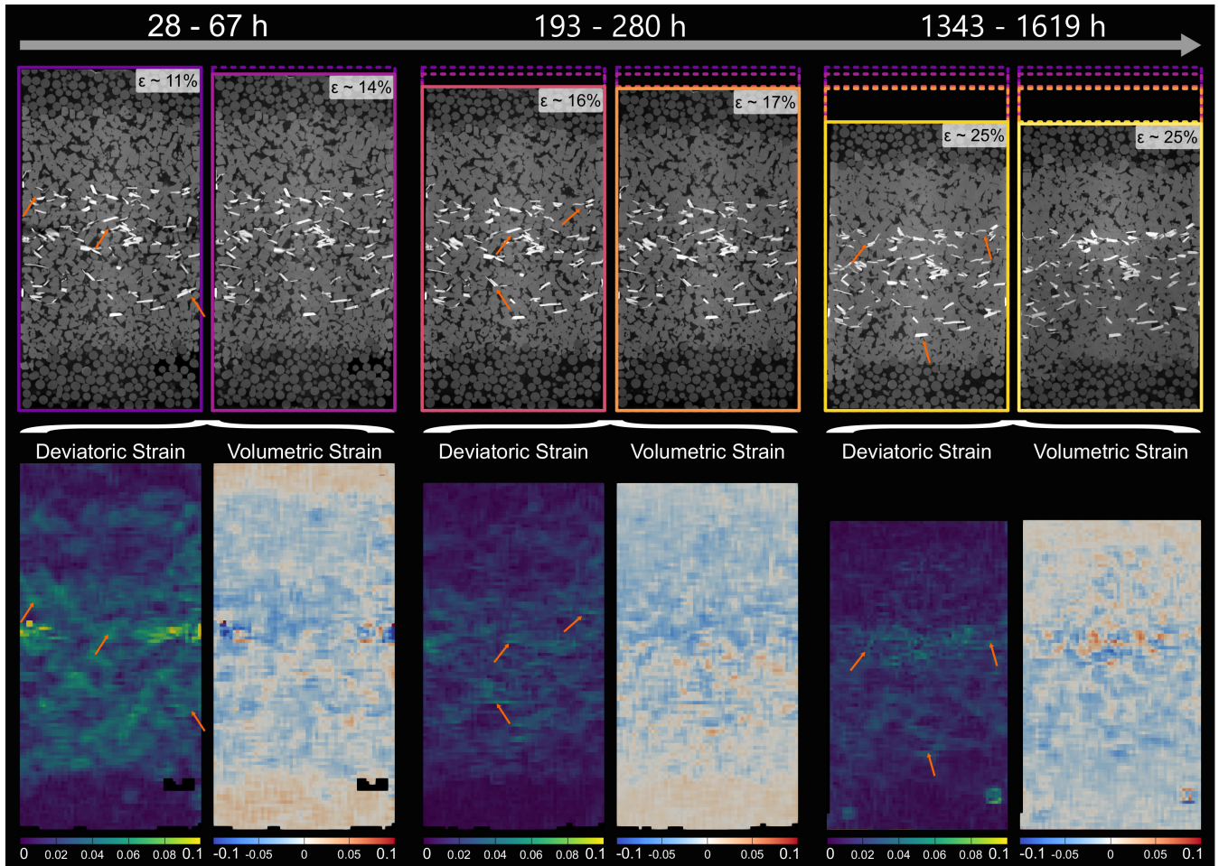
Figure 9. Locally resolved strain in the SBS sample . The absolute values of deviatoric and volumetric strain were calculated from digital volume correlation for three different time steps. The top row shows the two microtomography scans which were compared to each other using digital volume correlation. Further, the contours are showing the sample dimensions, ranging in colour from purple for the least compacted sample to light yellow for the most compacted sample . In the bottom row, the results of the strain calculation are displayed. Note that the strains are cumulative and cover the entire time interval between the two selected scans. The duration of the time intervals increase from the left to the right and are 39 hrs, 87 hrs and 276 hrs. For the deviatoric strain bright colours represent high strains whereas dark colours represent low strains. For the volumetric strain blue indicates compaction while red indicates dilation. Note that the strains are resolved on the grain scale. Arrows point to high deviatoric strains at NaCl-biotite interphase boundaries .
