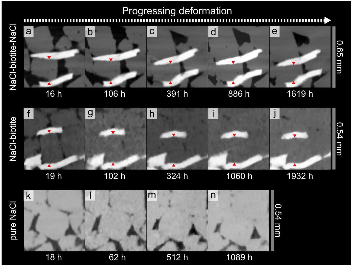
Figure 6. Sequence of time steps showing active dissolution-precipitation creep at the interphase boundaries of a NaCl grain-grains with two biotite grains in the SBS (a-e) and SB sample (f-j). While the size of the NaCl grains are reduced without showing any signs of brittle deformation, interphase contacts with the mica become flattened, indicating dissolution of NaCl. Comparison of a & e and f & j shows that the vertical strain accommodated by the NaCl grain-grains is \sim 26\% in the SBS sample and contacts with \sim 22\% in the micas flattened, indicating dissolution of NaCl SB sample. Note that the biotite grains have experienced only little rotation during deformation although 1603 hrs and 1913 hrs of compaction are in between the first and the last image images. The In the SBS sample, the rotation of the top biotite grain occurs pre-steady prior to the apparent steady state. Red arrows in a & e are used as markers for strain calculations. The pure NaCl sample (k-n) on the other hand shows less activity of DPC. However, here as well contacts between grains are flattened and pore space reduced.
