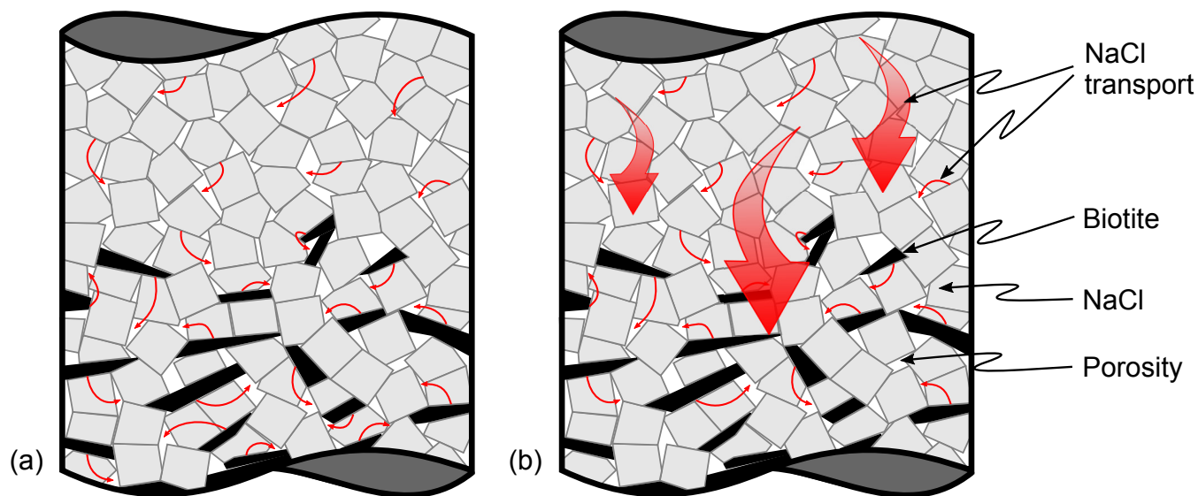
Figure 17. Possible transport length scales during dissolution-precipitation creep as proposed with-in-within the scope of this work. In a) Diffusion occurs only on the grain scale as described in the classical literature. In b) we added diffusive transport on longer length scales as described in Merino et al. (1983). However, diffusive transport on the grain scale is considered to be active as well.
