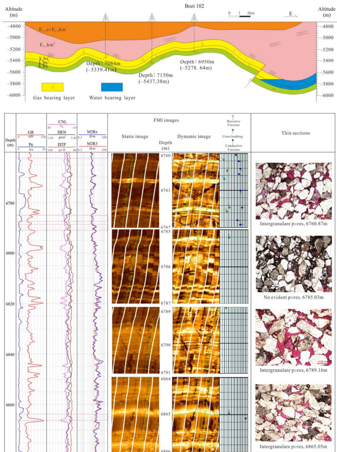
Figure 21. Cross-section of Bozi 1-Bozi 101-Bozi 102 and pore spaces as well as fractures determined from thin section and image logs for Well Bozi 102
