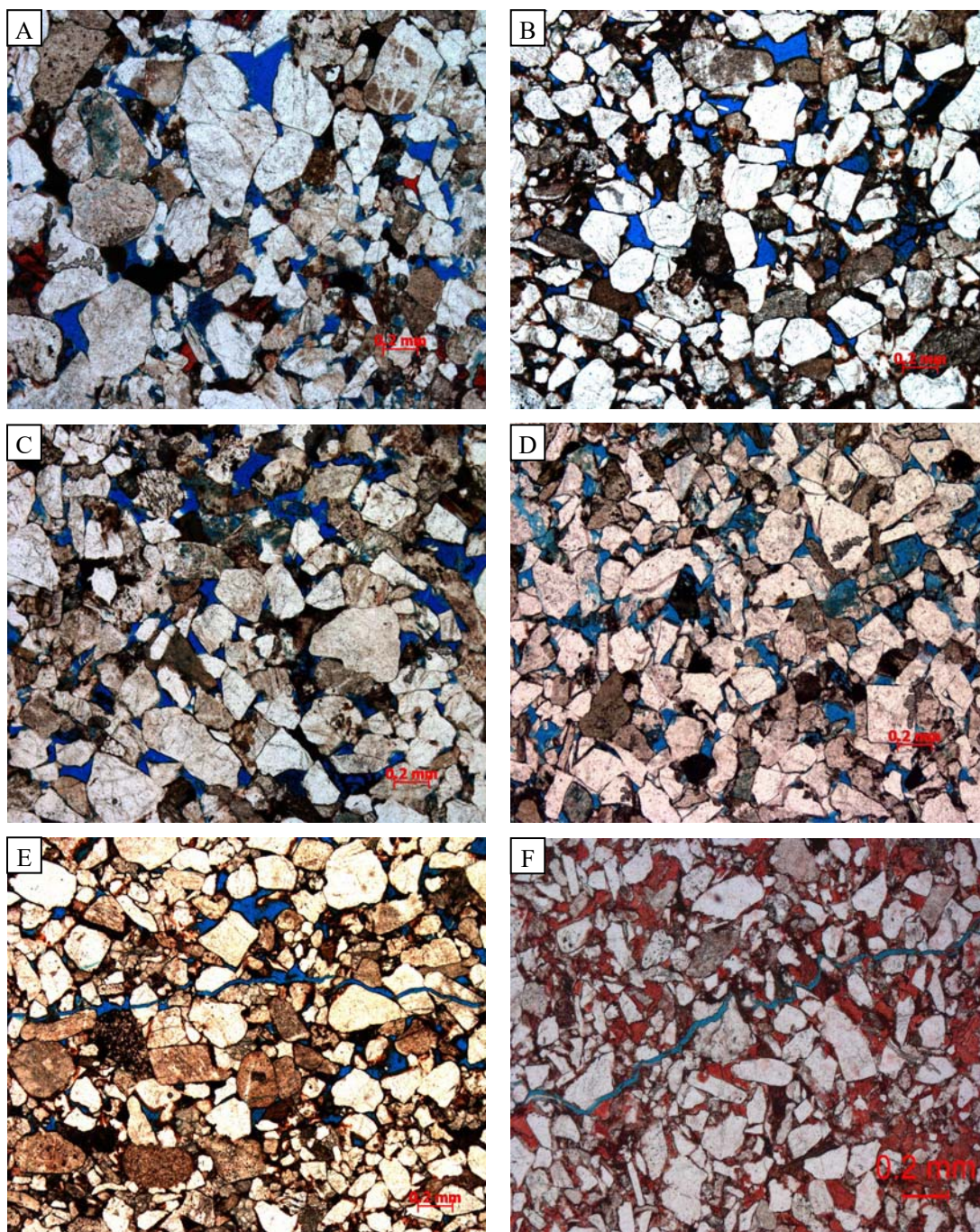
Figure 4. Thin section images showing the pore spaces of Cretaceous Bashijiqike Formation in Kuqa Depression
