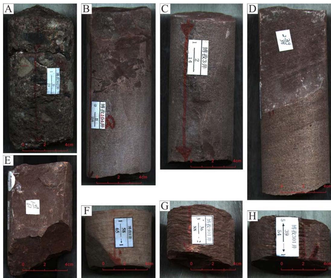
Figure 3. Core photos showing the lithologies of Cretaceous Bashijiqike Formation in Kuqa Depression
