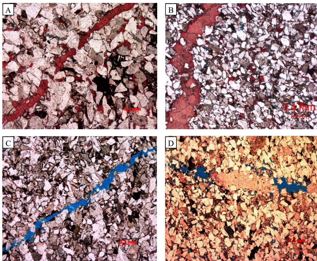
Figure 11. Thin sections showing the cementation and dissolution along the fracture surfaces of Cretaceous Bashijiqike Formation in Kuqa Depression
