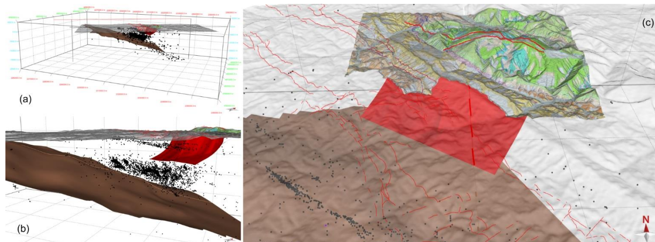
310 Figure 9: 3D model with DTM with wrapped geological map of the study area, showing relationships among normal fault system (red), ATF (brown) and earthquakes foci (black crosses). Detailing the model from a to c (see wind rose for orientation).
