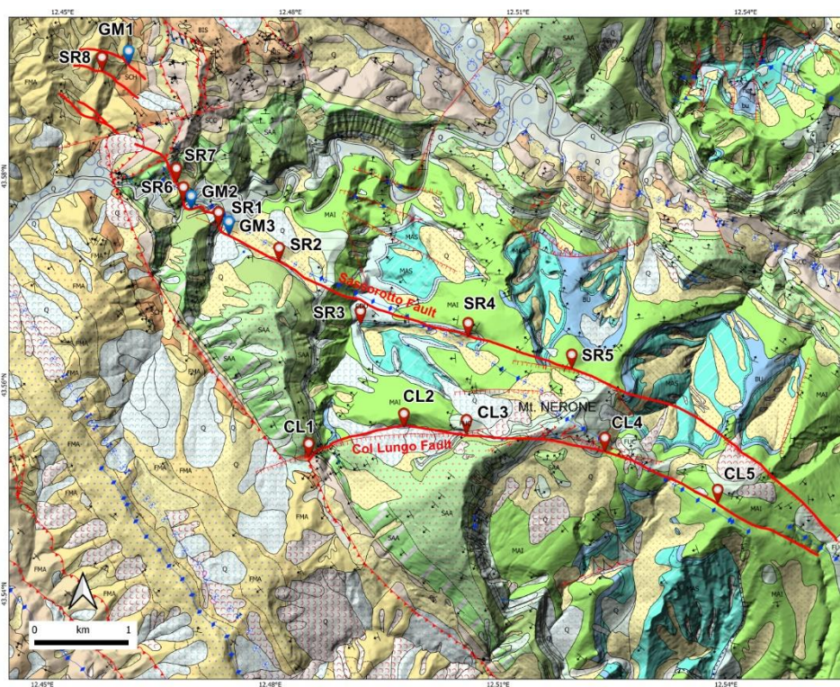
75 Figure 2: Simplified geological map of the study area from a geological map of the Marche region at a scale of 1:10,000 (Regione Marche, Carta geologica regionale 1:10,000, 2020). The thick red lines are the fault traces mapped in this study. SR (Sassorotto), CL (Col Lungo) and GM (Geomorphology) are the observation sites. Geological units: MAS, Calcare Massiccio Formation; BU, Bugarone Group; COI, Corniola Formation; RSA, Rosso Ammonitico Formation; POD, Posidonia Formation; CDU, Calcari diasprini; MAI, Maiolica Formation; FUC, Fucoidi Marls Formation; SBI, Scaglia Bianca Formation; SAA, Scaglia Rossa Formation; VAS, Scaglia Variegata Formation; SCC, Scaglia Cinerea Formation; BIS, Bisciaro Formation; SCH, Schlier Formation; FMA, Marnoso Arenacea Formation; Q, Quaternary deposits.
