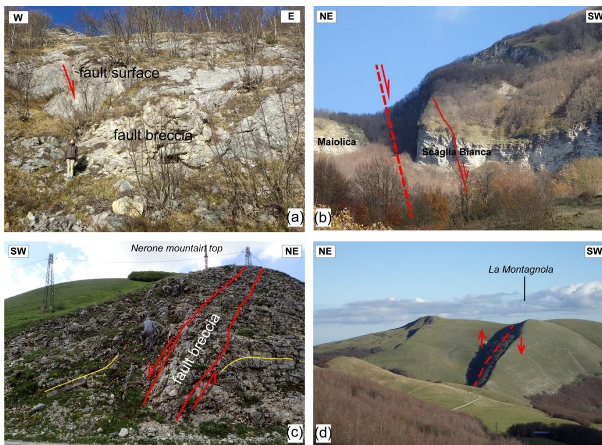
195 Figure 5: Col Lungo Fault (sites location in Fig. 2). (a) site CL2- large outcrop where fault surface and related breccias are well exposed. (b) site CL3- the older Maiolica Fm in the footwall is separated by a deep gorge to the Scaglia Bianca Fm in the hanging wall cut by a minor synthetic fault. (c) site CL4- normal fault in the Maiolica Fm outcrops on the road cut nearly on top of the mountain showing a fault breccia and drag folds in the footwall. (d) site CL5- interpreted prolongation of the fault along the ridge doubling on top of Montagnola Mt.
