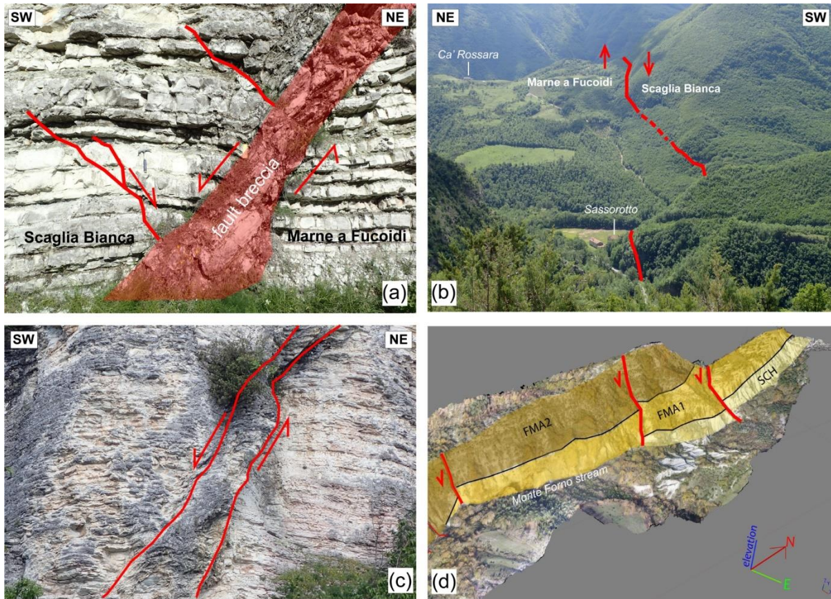
110 Figure 4: Sassorotto Fault (site location in Fig. 2). (a) site SR1- fault outcropping at Sassorotto locality showing a large thickness of breccia and an antithetic minor fault. (b) site SR2- the morphological scarp shows a height inversion where younger Scaglia Bianca Fm is move down to the older Marne a Fucoidi Fm (c) site SR6- fault on the outcrop at Biscubio river. (d) site SR8- the terrigenous facies of Marnoso Arenacea Fm and their relative movements respect to the interpreted faults is showed on the photo-mosaic (draped on DEM built by drone data collection).
