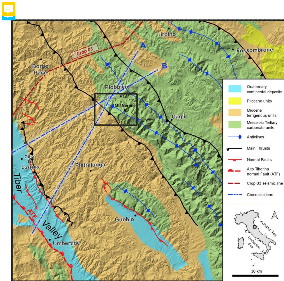
Fig. 1: Schematic tectonic map of the northern sector of the Umbria–Marche Apennines (northern Apennines), showing the study area by the black rectangle (Fig. 2) and the traces of the cross-sections (Fig. 10).
