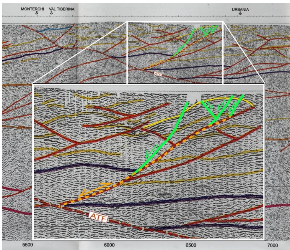
285 Figure 7: Reinterpreted Crop-03 seismic reflection profile (Barchi et al., 1998) close to the study area. On the buried crestal sector of the Monte Nerone anticline, some extensional feature of the reflectors can be interpreted as normal faults (green) similar to the ones outcropping in the study area and their relationships with negative inversion movement (orange) on the deeper thrust ramp. ATF: Alto Tiberina Fault.
