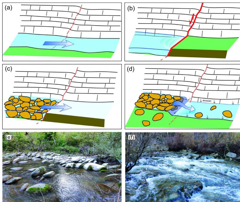
255 Figure 6: Whitewater evolution model by faulting, deposition and erosion. (a) pre-faulting possible situation; (b) fault movement developing a countercurrent step; (c) boulders are deposited against the fault footwall where flow energy is lower; (d) fluvial erosion eliminated the fault wall, but the boulders (even if some of them are carried downstream) became the step originating whitewater; (e) imbricated boulder deposits on the hanging wall on the Biscubio river; (f) step of boulders producing present whitewater.
