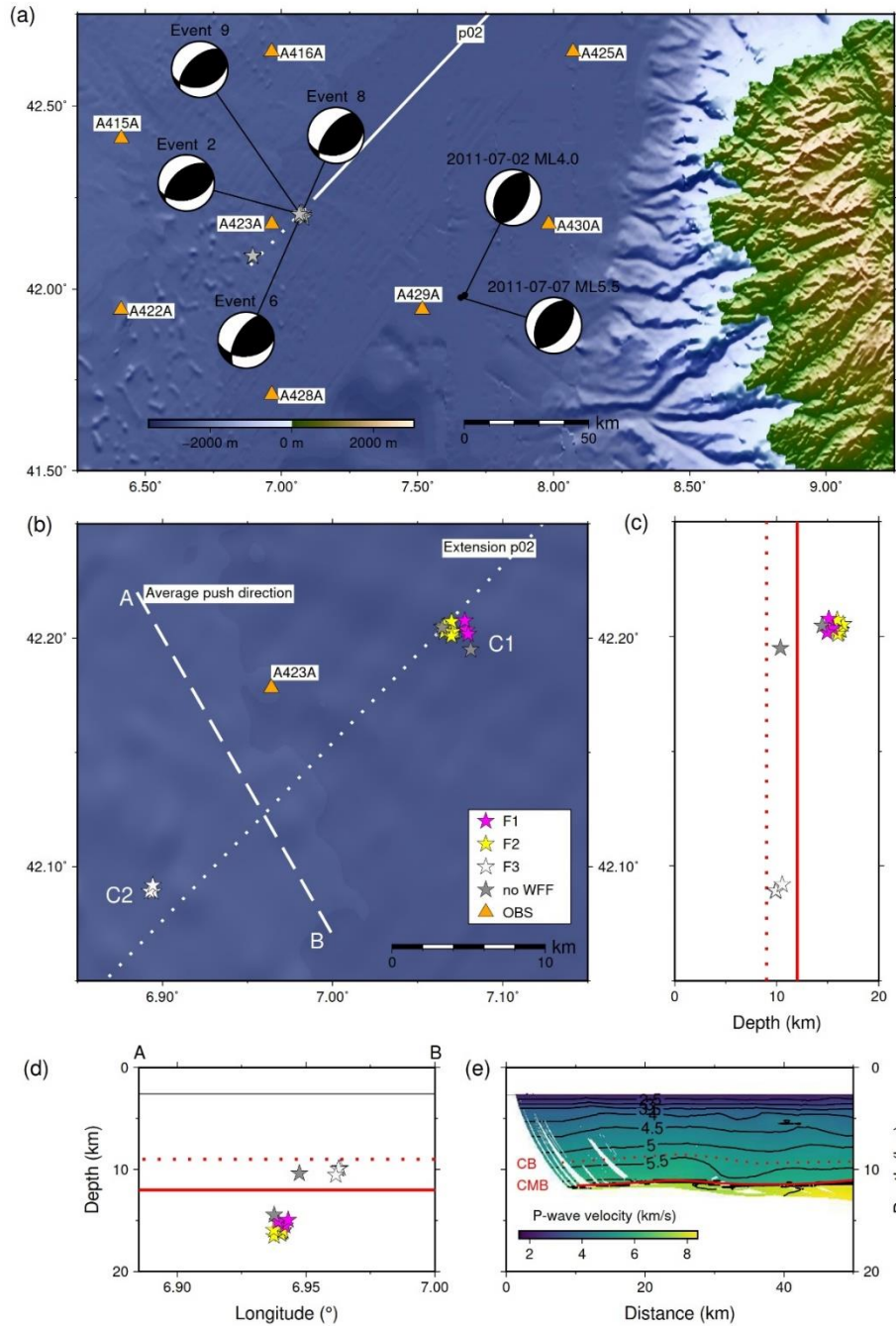
260 Figure 5: (a) Focal mechanisms of C1 cluster and two events in 2011 (Larroque et al., 2016). (b) Zoom into the map from panel a. The white dotted line indicates the prolongation of seismic refraction profile p02 (white line in panel a) and the white dashed line represents the main horizontal direction of the pressure axis P as indicated by focal mechanisms. Events are displayed coloured according to their wave form family (WWF). (c) Depth distribution of the cluster events from North to South. (d) Events projected on the dashed line A-B shown in panel b. The thin black line indicates the seafloor, the dotted red line is the base of the sediment 265 layers (CB) and the solid red line is the crust-mantle boundary (CMB). (e) SW end of the seismic velocity model computed from seismic refraction profile p02 (Dannowski et al., 2020). Topography from GMRT data (Ryan et al., 2009).
