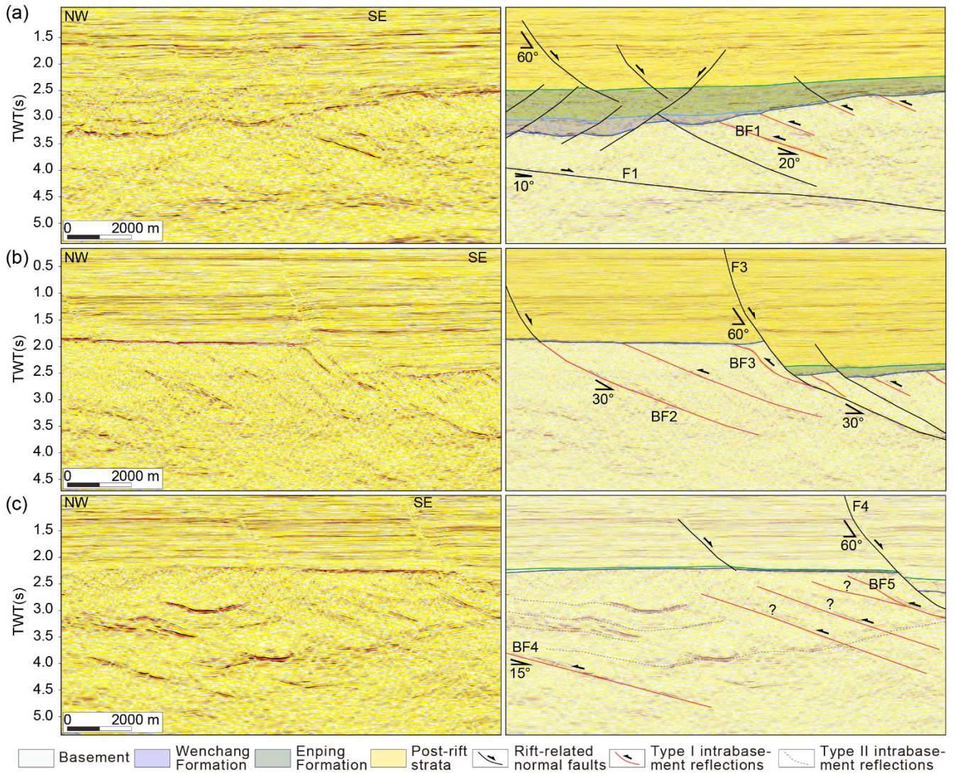
Fig. 5 Uninterpreted (Left panels) and interpreted (Right panels) cross-sections showing the occurrence of intrabasement structures in the study area. (a) and (b) show the characteristics of Type I intrabasement structure, while (c) shows the interpretation of Type II intrabasement structure with Type I intrabasement structure. Question mark indicates uncertainty of the interpretation. See Fig. 1 for location. Colours within the sedimentary cover correspond to ages shown within the stratigraphic column (Fig. 2)
