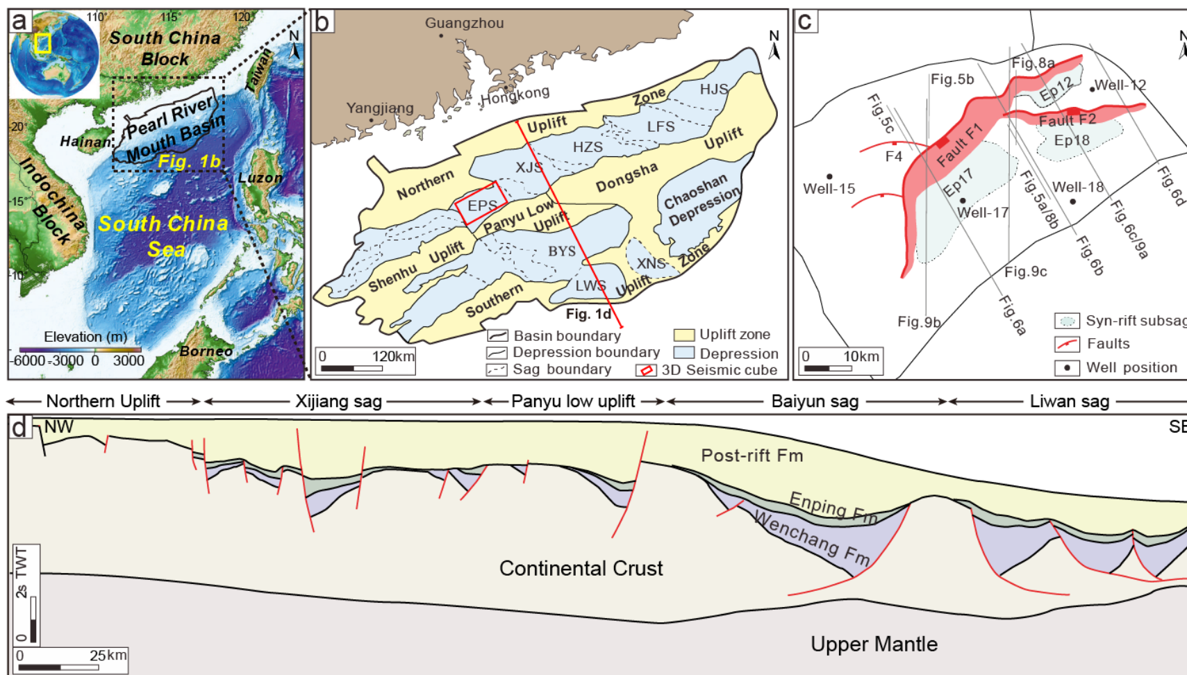
Fig. 1 Location and simplified structural map of the study area. (a) Topography and bathymetry of the South China Sea and adjacent regions. (b) Map of structural divisions of the Pearl River Mouth Basin and location of the Enping Sag. EPS—Enping Sag; XJS—Xijiang Sag; HZS—Huizhou Sag; LFS—Lufeng Sag; HJS—Hanjiang Sag; BYS—Baiyun Sag; LWS—Liwan Sag; XNS—Xingning Sag. (c) Schematic structural map and depocenter of the Enping sag at the basement. Straight lines show the location of cross-sections. (d) Transect across the middle part of the Pearl River Mouth Basin, showing the geological interpretation of the structure of the northern South China Sea margin. After Yang et al. (2018); Ye et al. (2018).
