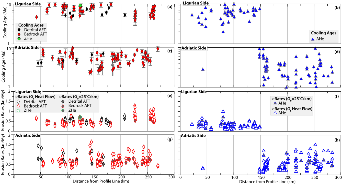
340 Figure 7 Profile parallel to the orogen strike (profile location shown in Fig. 3a) illustrating cooling ages along the Ligurian side for (a) AFT and ZHe data and (b) AHe data, and along the Adriatic side for (c) AFT and ZHe data and (d) AHe data. Erosion rates along the Ligurian side for (e) AFT and ZHe data and for (f) AHe data, and along the Adriatic side for (g) AFT and ZHe data and for (h) AHe data. In (d), individual AHe symbol dated to <1 Ma is illustrated with a double gray slash.
