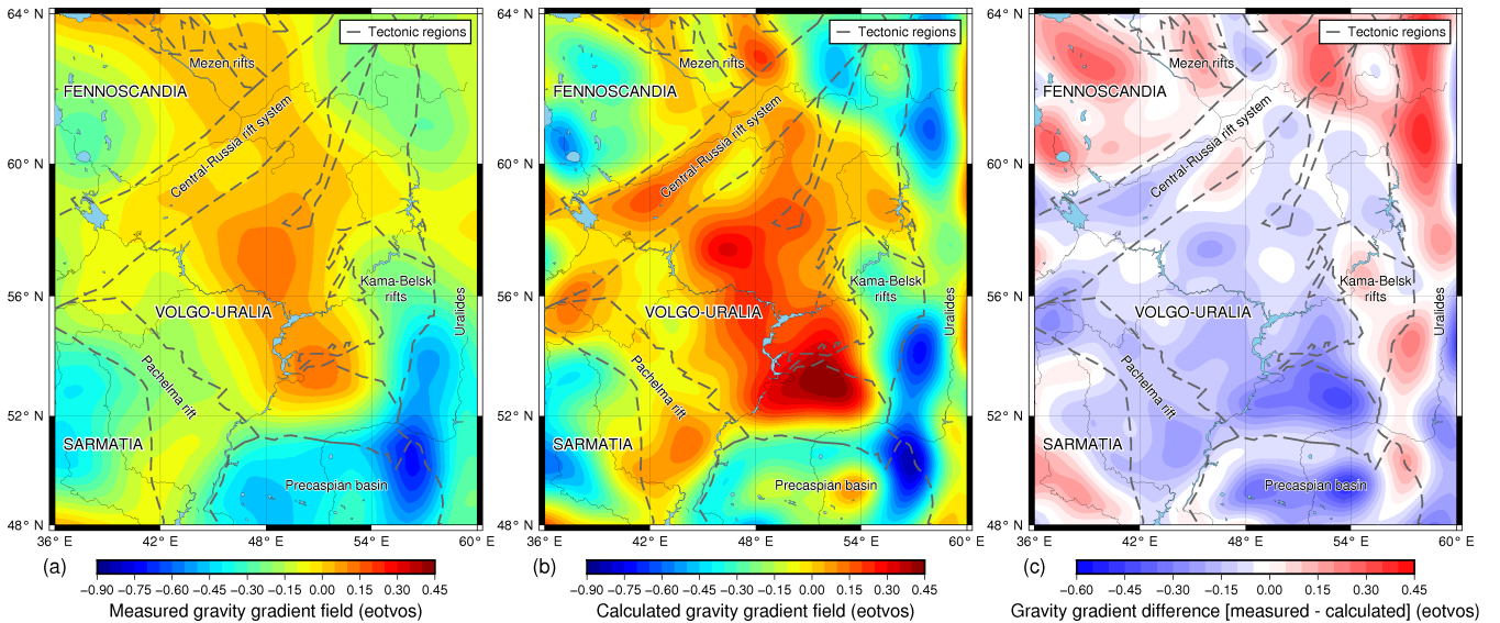
Figure 7: Comparison between measured and calculated gravity gradient fields. (a) GOCE topographically corrected vertical gravity gradient at 225 height (Bouman et al., 2016). (b) Calculated topographically corrected vertical gravity gradient field from IGMAS+ 3D model. (c) The difference between measured and calculated gravity gradient fields.
