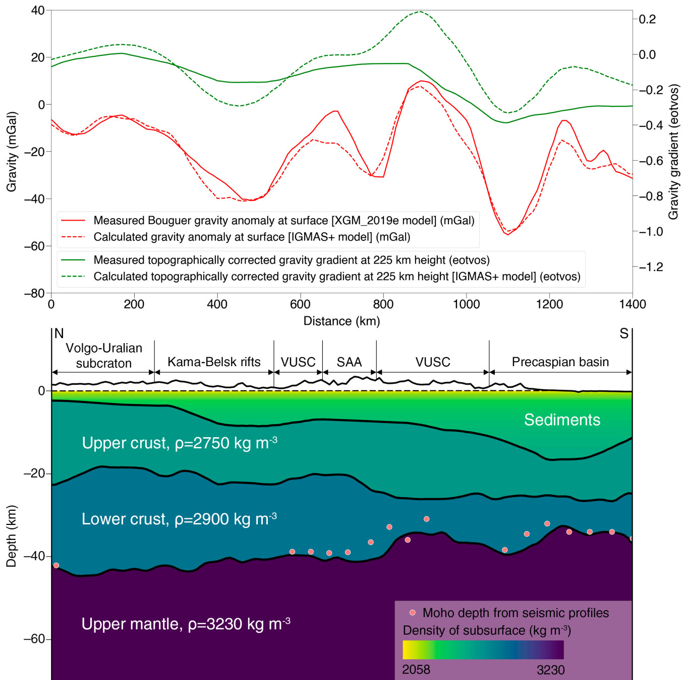
435 Figure 13: Measured and calculated Bouguer gravity anomalies and the topographically corrected vertical gravity gradient anomalies from the crustal model (top) and IGMAS+ model north-south cross-section in the eastern part of Volgo-Uralia (bottom) – see figure 3 for the reference on the map. Subsurface is vertically exaggerated by the factor of 10 and topography is by the factor of 100. VUSC stands for Volgo-Uralian subcraton and SAA for Sernovodsk-Abdulinsk Aulacogens.
