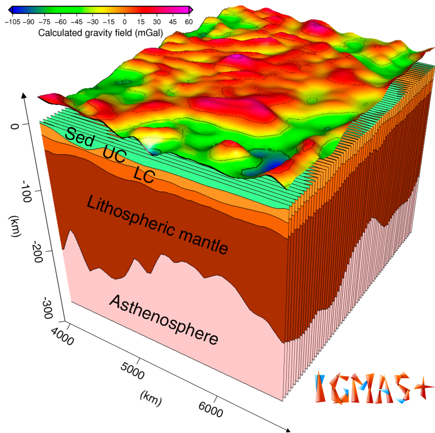
370 Figure 8: A 3D lithospheric model of Volgo-Uralia developed in IGMAS+ software. It consists of 67 vertical sections which gives a spatial resolution of approximately 50 km. The model includes 5 main layers: sediments (Sed), upper crust (UC), lower crust (LC), lithospheric mantle, asthenosphere, and an additional 6 th layer of underplating. The Bouguer gravity anomaly produced by the model is shown on top.
