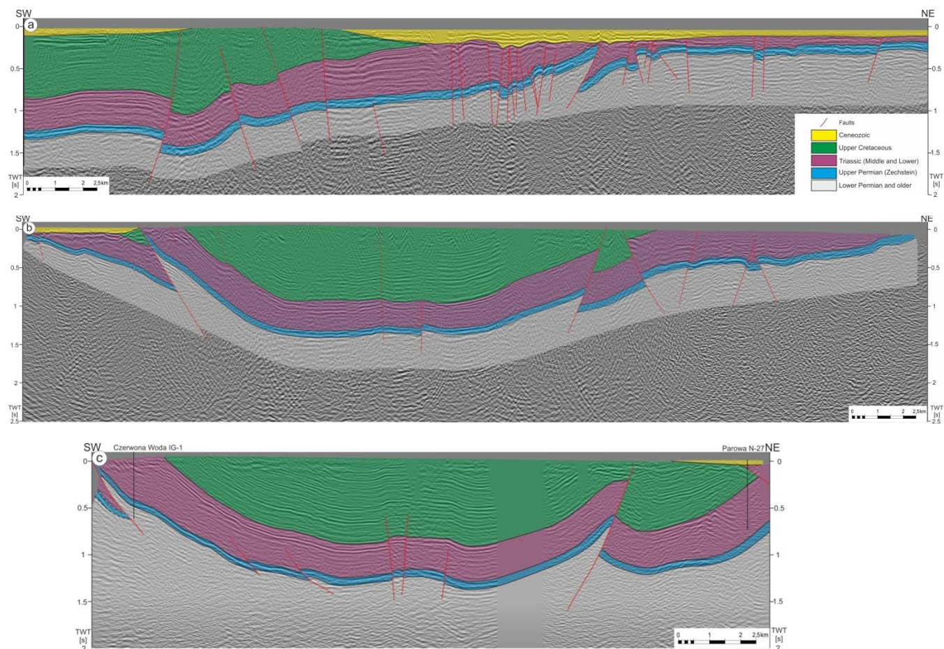
710 Figure 9 a-c: Interpreted seismic profiles from the North-Sudetic Synclinorium (location in Figure 6).
