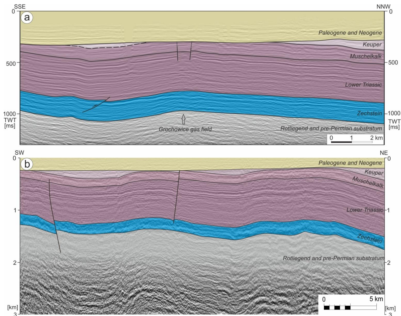
Figure 4: Two seismic profiles from the Fore-Sudetic Homocline (location in Figure 2) showing very gentle folds in Triassic and Permian (Rotliegend not marked). Note steep to low-angle mainly reverse faults. The anticlines are structural traps for hydrocarbons, with gas fields known in Rotliegend strata (e.g. Grochowice gas field in Figure 4a). Please note the different scales of the two profiles.
