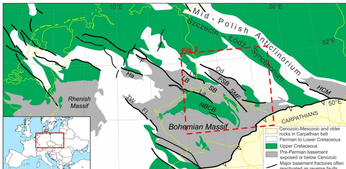
Figure 1: The main Late Cretaceous – Early Palaeogene tectonic structures in Central Europe. Modified after Kley and Voigt 2008.. Abbreviations: Lf - Lusatian Main Fault, Od - Odra Fault, Ha-Harz Block, F – Flechtingen High, TW - Thuringian Forest, FL – Franconian Line, LB - Lusatian Block, SB - Sudetic Block, FSB - Fore-Sudetic Block, NBCB - North Bohemian Cretaceous Basin, HCM - Holy Cross Mountains
