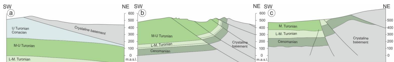
Figure 19: Schematic sections across the Lusatian Thrust in three localities, showing along-strike structure changes (based on Coubal et al., 2014). Location in Fig. 2.
