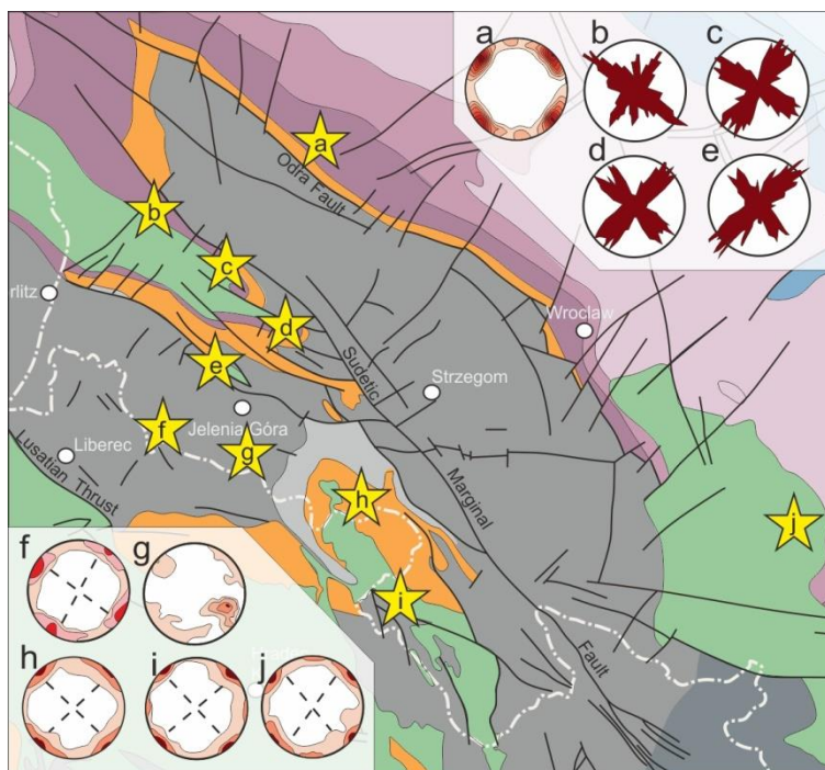
Figure 20: Comparison of stereograms and rose diagrams of the dominant steep joint sets coming from several local studies (by Jerzykiewicz et al., 1974, Aleksandrowski, 1976, Solecki, 2011, Selerowicz et al., 2014) made at various locations in the Polish Sudetes. Background: the geological map of Figure 2.
