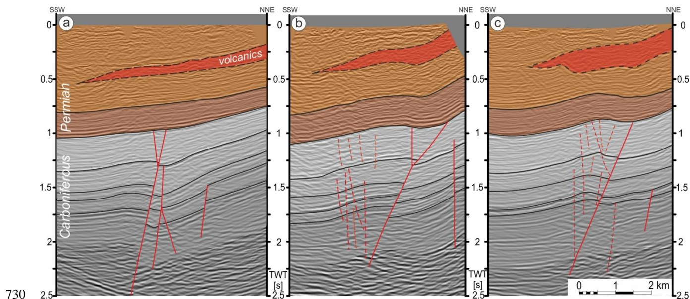
Figure 13: Seismic profiles from Mieroszów vicinities showing probable effects of Late Cretaceous – Early Palaeogene reactivation of a Carboniferous flower structure. The Permian volcanic member (red) continues to the NNE to outcrop massively in the Suche Mountains. Location is given in Figure 12.
