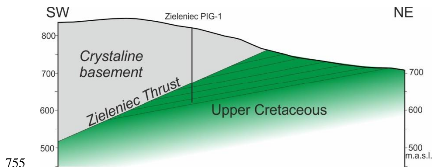
Figure 17: Schematic section across the Zieloniec Thrust (based on data from Cymerman, 1990, and Kozdrój, 2014). Location in Fig. 12.
