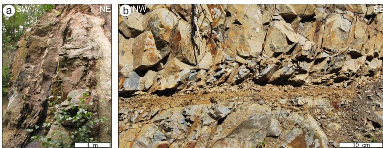
Figure 18: Examples of outcrop-scale brittle structures related to major faults at the SW boundary of the Intra-Sudetic Synclinorium.
