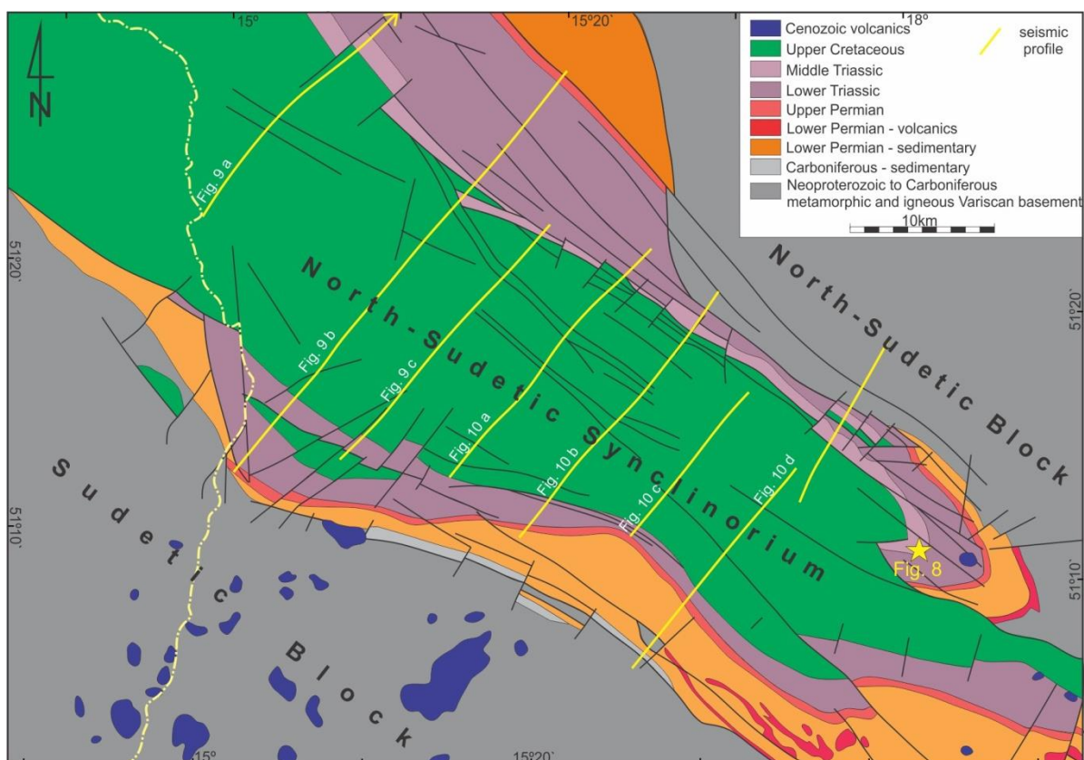
Figure 6: Geological map of the North Sudetic Synclinorium (based on Balazińska and Bossowski, 1979; Krentz et al., 2001 and Cymerman, 2010). Locations of interpreted seismic profiles are shown. For full-length location of seismic profile of Figure 8a - see Figure 2. The map is based on Solecki (1994) and Cymerman (2010).
