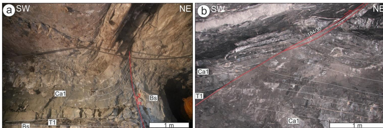
Figure 5: Examples of tectonic structures observed on galleries' walls in copper and silver mines on the Fore-Sudetic Homocline at the base Zechstein ore-bearing formation (location in Figure 2). (a) Inverted steep fault, originally normal. The inversion caused fault-drag of Ca1 Zechstein Limestone. (b) Thrust fault in carbonate rock. Abbreviations: Bs- Weissliegend Sandstone, T1-Kupferschiefer Shale, Ca1-Zechstein Limestone.
