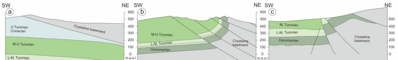
Figure 19: Schematic sections across the Lusatian Thrust at three localities, showing along-strike stucture changes (based on Coubal et al., 2014). Location in Fig 2.
