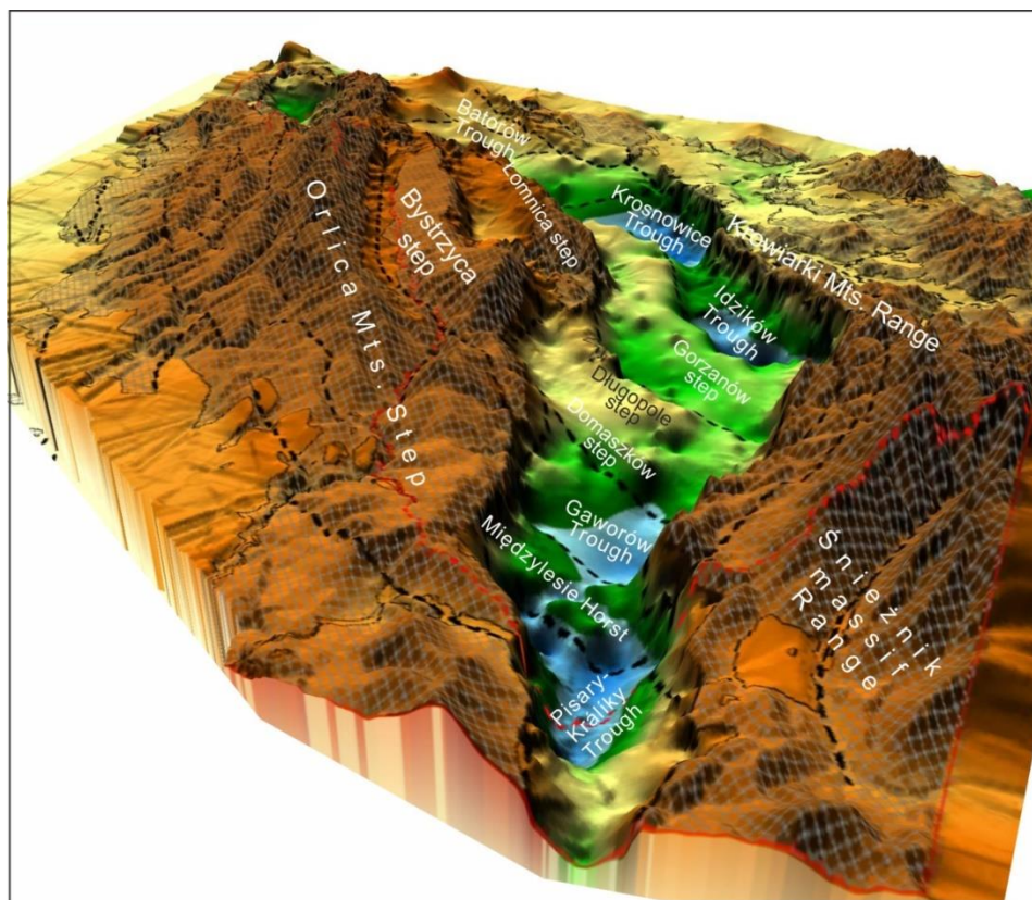
Figure 15: Perspective view towards the north onto the base Cretaceous relief (known from boreholes) in the Upper Nysa-Králiký Graben (from Badura and Rauch, 2014). The oblique-striking troughs, steps and horsts reflect NW-SE trending Late-Cretaceous – early Palaeogene structural grain defined by inverted blocks underlying the Cretaceous graben floor and folds in its fill (removed from the picture), once continuing laterally, before the graben formed in Miocene times. Location given in Fig 2.
