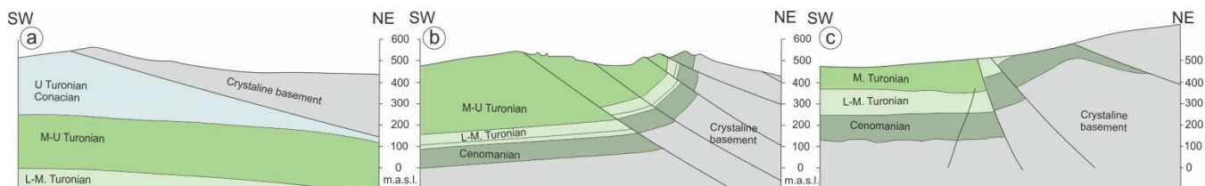
Figure 18: Schematic sections across the Lusatian Thrust at three localities, showing along-strike stucture changes (based on Coubal et al., 2014). Location in Fig 2.
