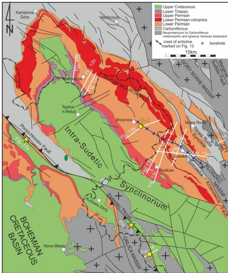
830 Figure 11: Geological map of the Intra-Sudetic Synclinorium (based on Grocholski and Augustyniak, 1971, Bossowski and Ihnatowicz, 2006, and Cymerman, 2010). Location of the interpreted seismic profiles and described localities is shown. CZT – Czerwieńczyce Trough (reverse graben).
