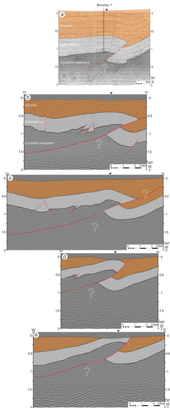
Figure 13: Seismic profiles (paper print version – Brada et al., 1982) from vicinity of Broumov (a) and from vicinities of Radków (b-e). Location in Fig. 11. The section (a) shows that the Broumov well was drilled in the hanging-wall of a thrust fault and, hence, the Carboniferous in the neighbourhood may occur deeper than found in the well. The thrust continues to the NE parallel to the bedding – most probably along the Lower Permian Anthracosia Shale member.
