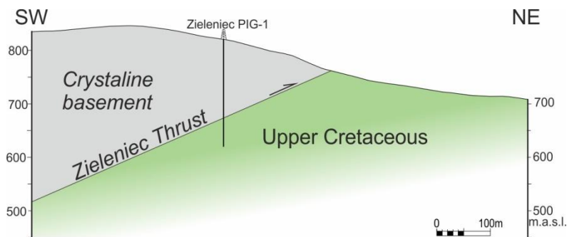
Figure16: Schematic section across the Zieloniec Thrust (based on data from Cymerman, 1990, and Kozdrój, 2014). Location in Figs 2 and 11.
