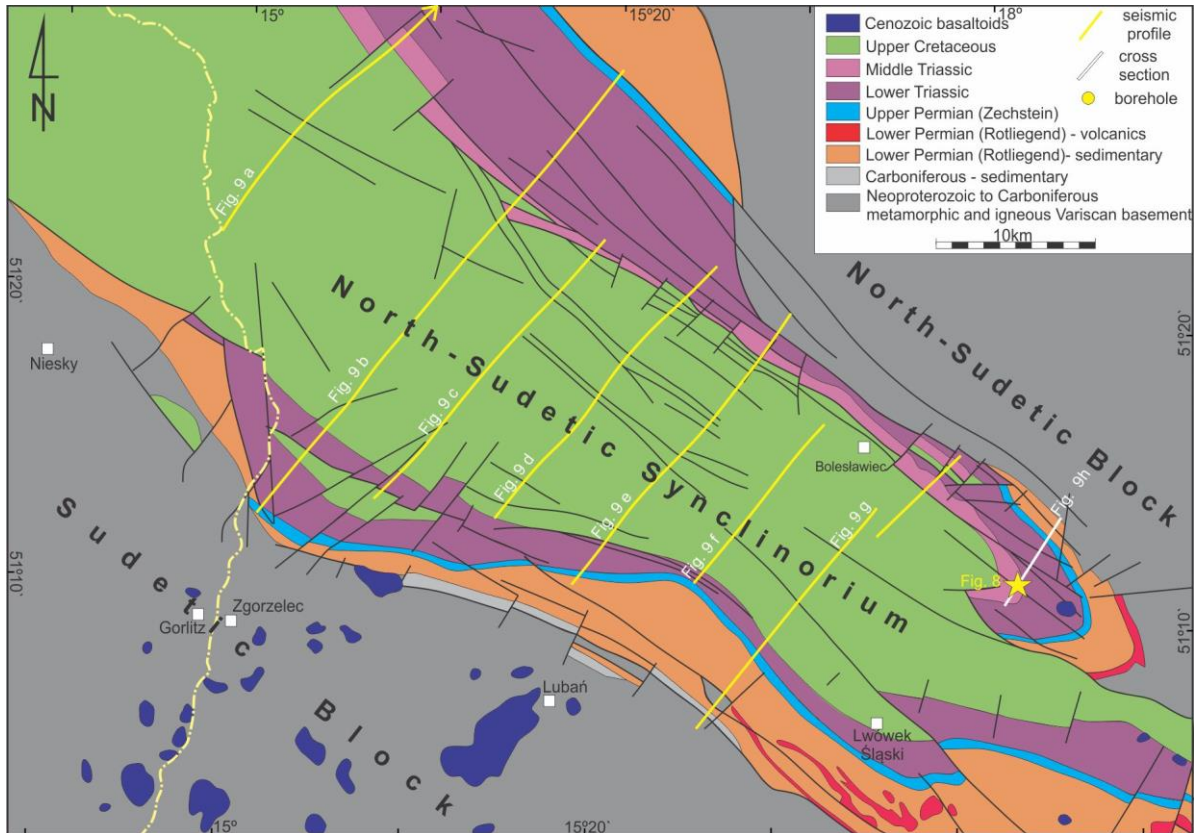
Figure 6: Geological map (without Cenozoic) of the North Sudetic Synclinorium (based on Bałazińska and Bossowski, 1979; Solecki, 1994; Krentz et al., 2001 and Cymerman, 2010), showing locations of the interpreted seismic profiles. For full-length location of seismic profile of Fig. 9a - see Fig. 2.
