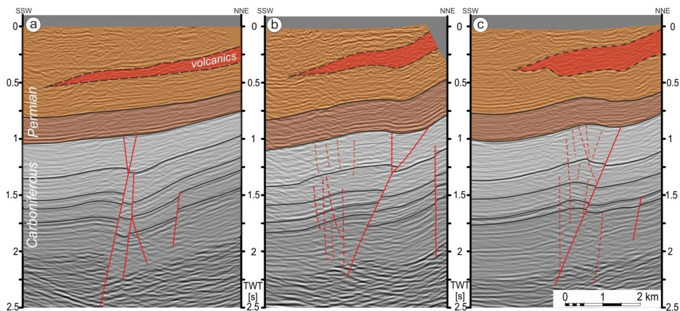
835 Figure 12: Seismic profiles from vicinity of Mioszów arranged successively along-strike of the structures, showing probable effects of Late Cretaceous – early Palaeogene reactivation of originally Carboniferous faults. The Permian volcanic member (in red) continues to the NNE to outcrop massively in the Suche Mountains. Location in Fig. 11. The faults in (a) do not show effects of post-Carboniferous reactivation, but further to SE the motion on faults resulted in very gentle folding of the overlying Permian strata.
