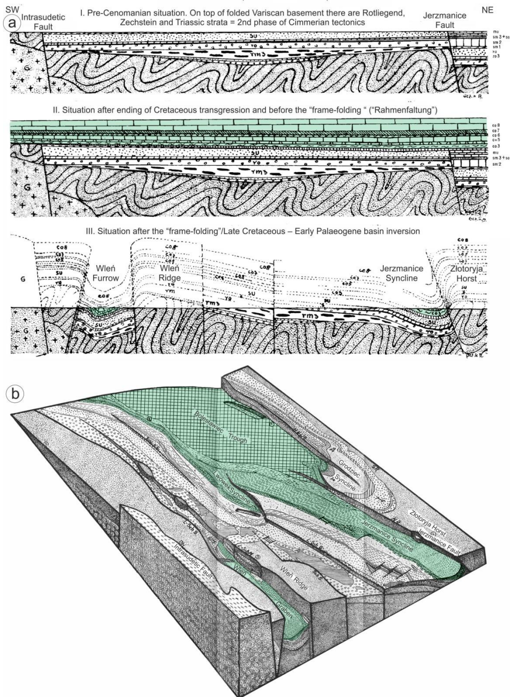
Figure 7: Kurt Beyer's (1939) interpretation of the "young Saxonian" tectonics in the North Sudetic Synclinorium (Basin). (a) Main tectonic deformation stages in the North Sudetic Basin. (b) Block-diagram showing simple open structure of the western part of the North Sudetic Synclinorium (Bolesławiec Trough) and complex pattern of blocks and synclinal grabens (Jerzmanice Syncline and Wleń Trough) in its eastern part (cf. Figs. 2 and 6).
