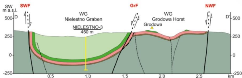
Figure 10: Simplified geological map and three selected cross-sections of the Wleń Graben according to Kowalski (2020)
