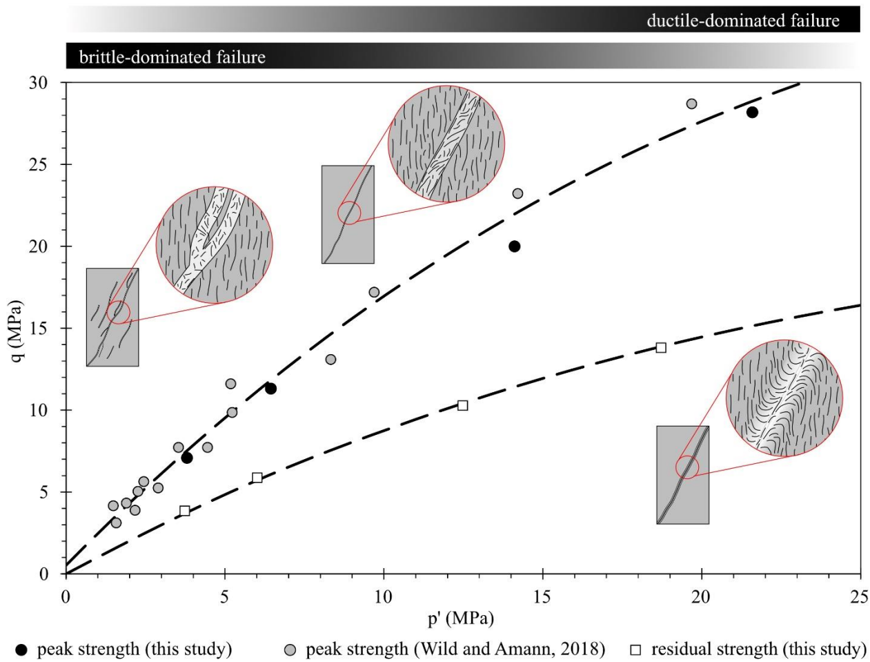
Figure 11: Peak and residual effective strength of shaly Opalinus Clay under triaxial undrained compression and our microstructural model for shear failure. The non-linear failure envelopes, fitted through all data points, underlines the gradual transition for deformation microstructures from brittle to ductile and the tendency for suppression of dilatancy due to the reduction in shear zone porosity.
