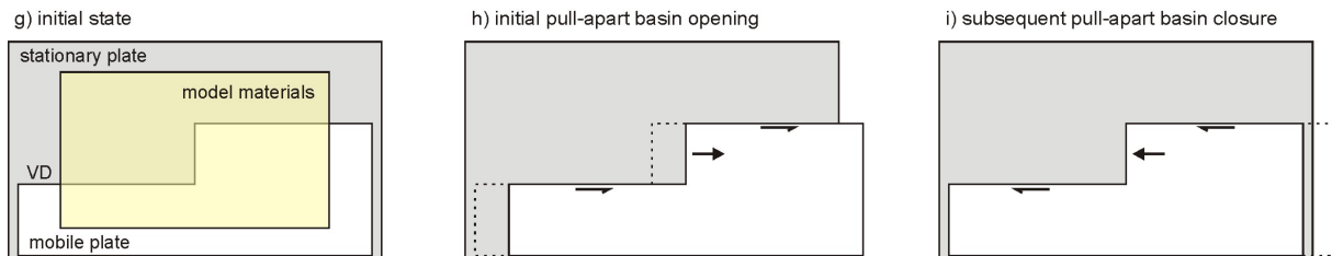
Figure 6. Examples of 3D kinematics in basin inversion models. (a-c) Oblique inversion tectonics example. The plate motion direction is defined as angle \alpha , the angle between the normal to the model axis and plate motion direction (e.g. Zwaan et al., 2016; Brune et al. 2018, and references therein). VD: velocity discontinuity (mobile base plate edge). Based on Brun and Nalpas (1996). (d-f) Rotational inversion tectonics example. RA: rotation axis. Based on Jara et al. (2015, 2018). (g-i). Inverted pull-apart basin example. Based on Wang et al. (2017). Modellers have used a wide variety of other base plate geometries for basin inversion experiments (see section 3.3.).
