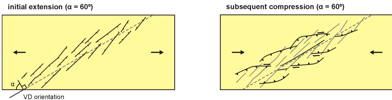
860 Figure 12. Top view of an inversion model involving a base plate set-up with brittle-viscous layering and (a) initial oblique extension leading to a series of en echelon normal faults, followed by (b) subsequent oblique inversion leading to (oblique) thrusting and strike-slip faulting. Inspired by Ustaszewski et al. (2005).
