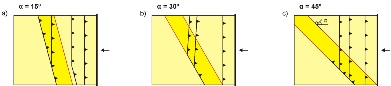
990 Figure 15. Effect of pre-existing graben orientation on fault reactivation during subsequent compression and inversion in brittle-only models, shown in map view. Grabens are indicated in yellow, and their orientation is defined as angle \alpha , angle between the normal to the graben strike and backstop motion direction. Image inspired by Yagupsky et al. (2008) and Deng et al. (2019).
