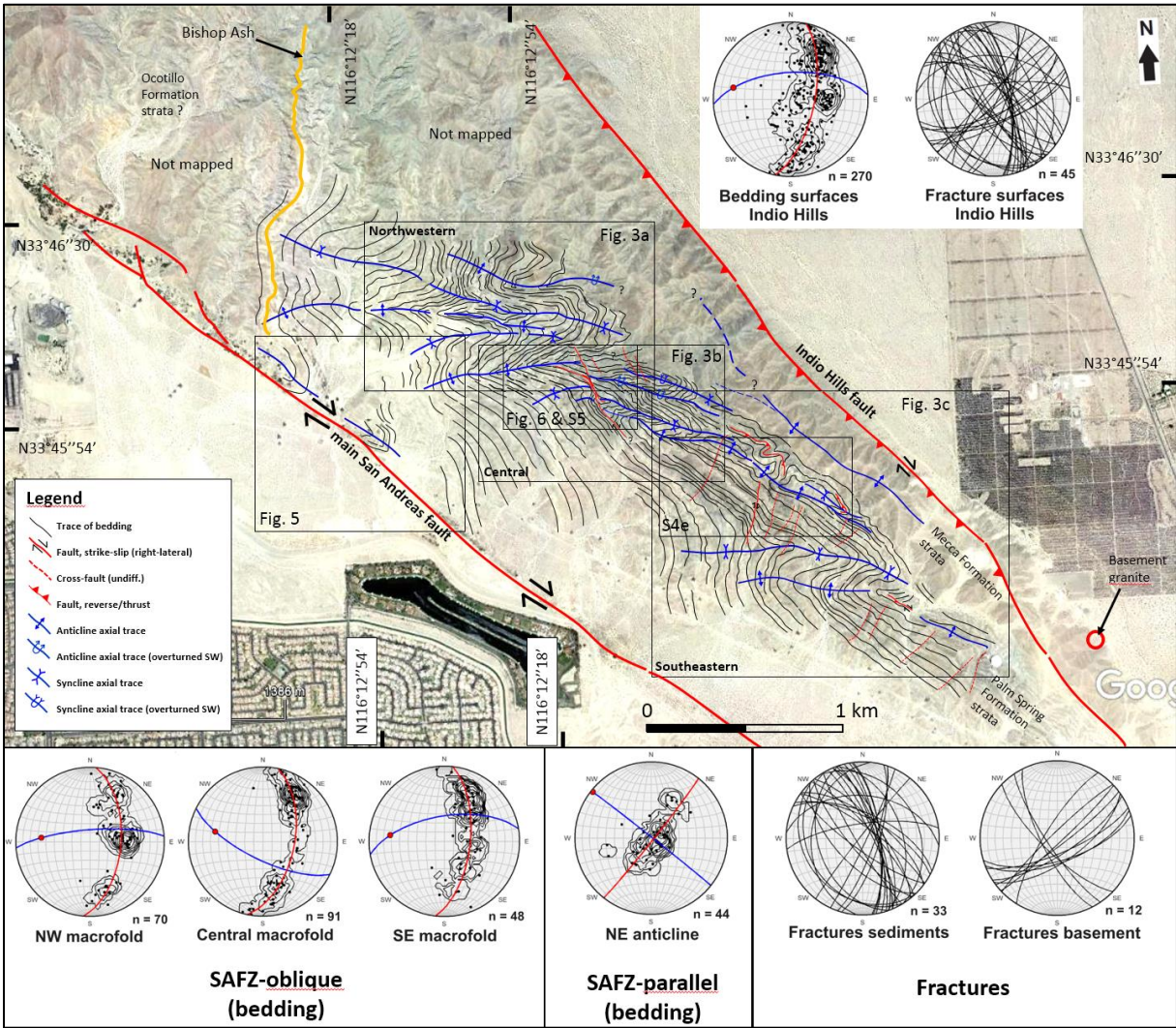
Figure 2: Interpreted DEM image in the southeastern part of the Indio Hills uplift area. Three main SAFZ-oblique macro-folds (northwestern, central, southeastern) are mapped in between the bounding Indio Hills and main San Andreas faults, whereas one SAFZ-parallel anticline is present close to the Indio Hills fault. More detailed figures are numbered and framed. Structural datasets are plotted in lower hemisphere Schmidt stereonet projections via the Orient software (Vollmer, 2015). Bedding surfaces are shown as pole to plane with frequency contour lines, with average \pi S great circle (red great circles), fold axial surface (blue great circles) and fold axis (red dots). Brittle fractures in sedimentary strata and basement rocks are plotted as great circles. Source: Google Earth historical imagery 09-2011. Uninterpreted version of the image available as Supplement S1. © Google Earth 2011.
