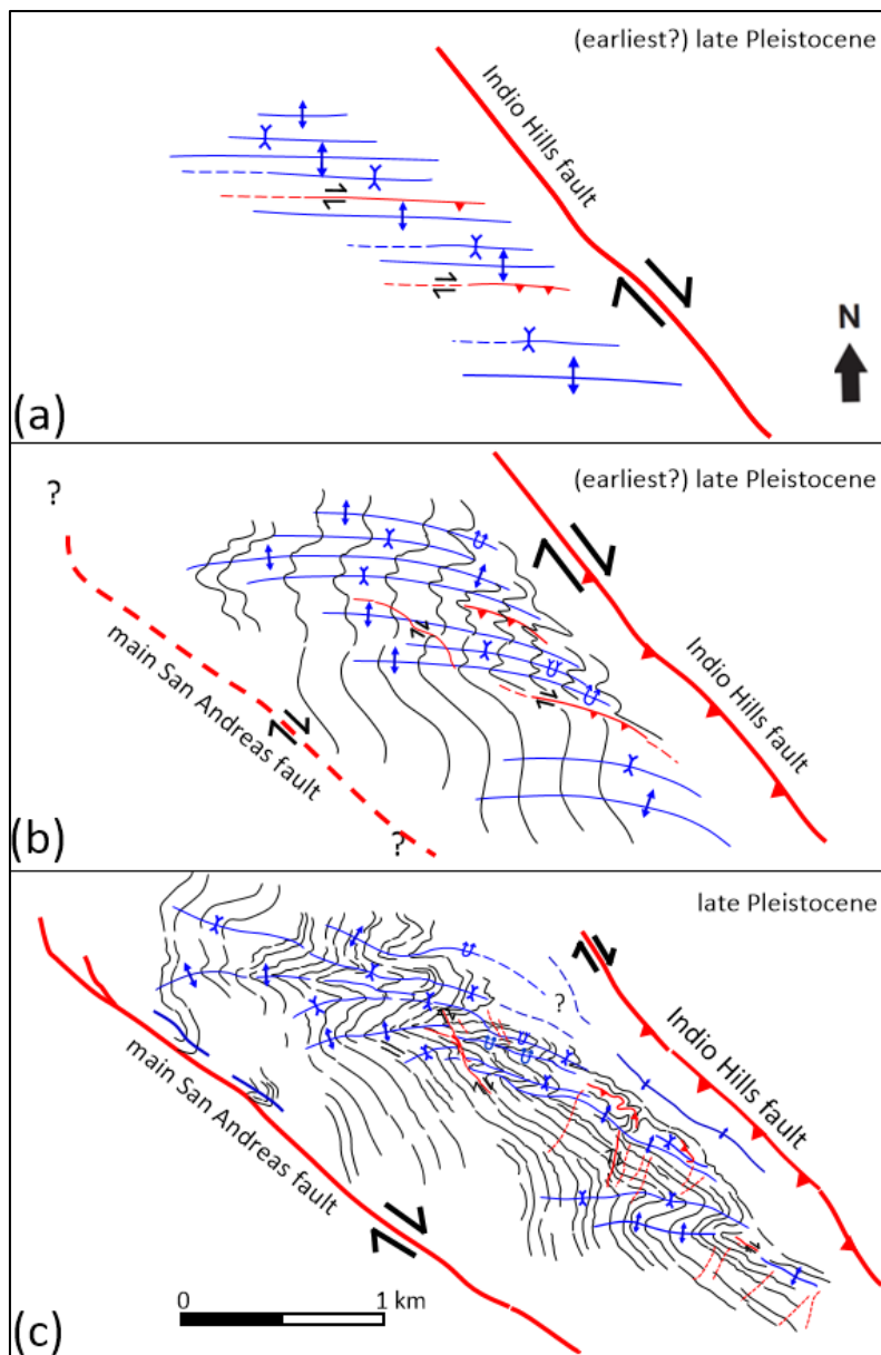
Figure 7: Model illustrating the progressive uplift/inversion history of the Indio Hills presuming a narrow time interval between formation of all structures in the area, except for the main San Andreas fault and associated folds. (a) Early distributed transpressional strain and formation of three major, en echelon oriented macro-folds, several subsidiary parasitic anticline-syncline fold pairs, and bed-parallel strike-slip and reverse (décollement) faults initiating at a high angle (c. 45°) to the Indio Hills fault. (b) Incremental partly partitioned transpression when the Indio Hills fault started to accommodate oblique-reverse movement forcing previous horizontal en echelon macro-folds and parasitic folds to tighten, overturn, and rotate into steeper westward plunges. Note also sigmoidal rotation of axial traces on the back-limbs of the macro-folds to low angle (< 20–30°) with the Indio Hills fault. (c) Late-stage advanced strain partitioning
